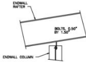
B6 ENDWALL RAFTER TO COLUMN
