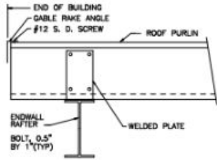
A7 SECTION THRU ENDWALL RAFTER
