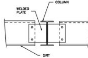
C6 GIRT TO COLUMN
