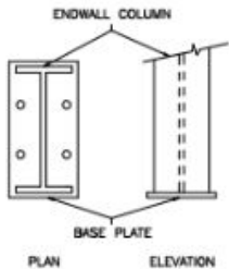
E3 BASE PLATE FOR ENDWALL COLUMN
