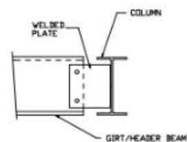
C15 GIRT/HEADER BEAM TO R/W COLUMN
