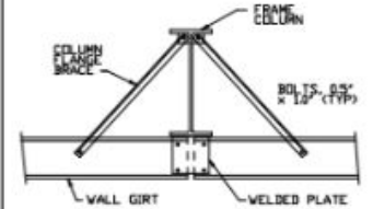
H4 WALL GIRT TO FRAME COLUMN
