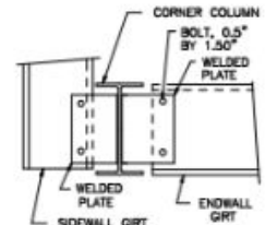
D6 CORNER COLUMN TO WALL GIRT
